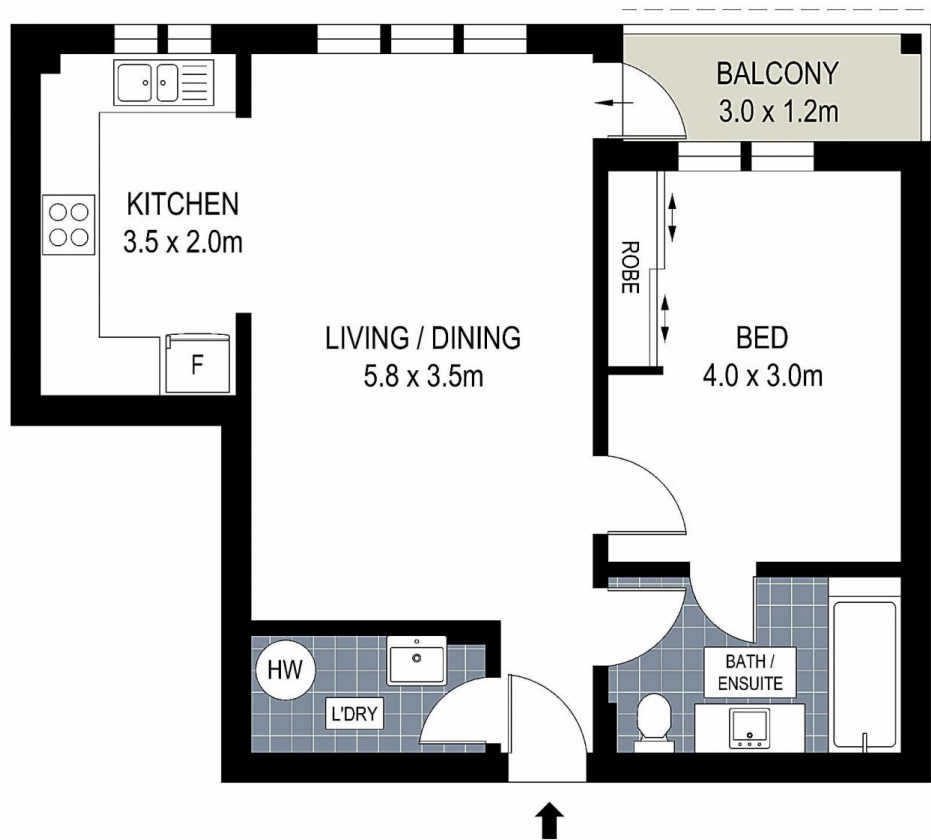
↑ TOP FLOOR / SECOND FLOOR
